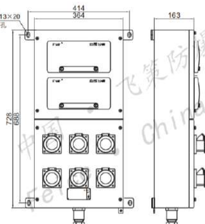
2型16A插销 2Type 16A latch
