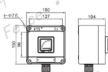
1型(挂式) Type 1 (hanging type)
