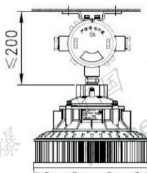
吸顶式(X)/配吊灯盒 Ceiling type(X)/ equipment chandelier box
