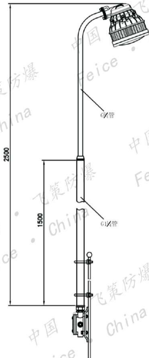
护栏式(C)安装 Installation of guardrail(C)
