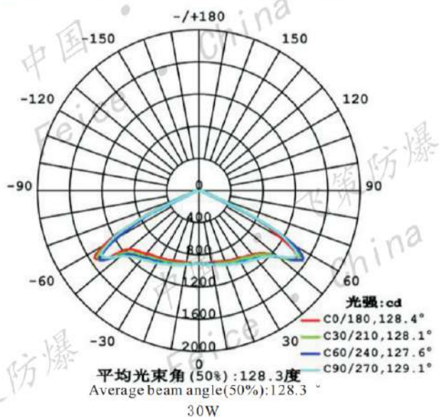
■ 配光曲线 Luminous distribution curve
