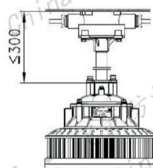
吊杆式(G)/配接线盒 Suspender type(G)/ equipment junction box
