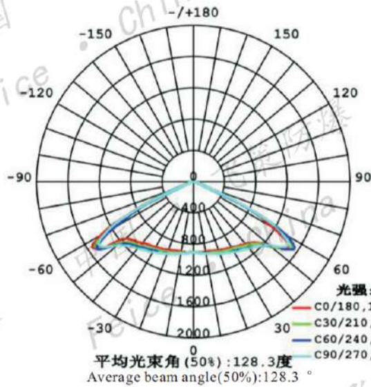
■ 配光曲线 Luminous distribution curve
