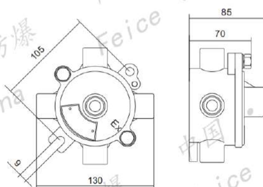
G1/2, G3/4, G1尺寸规格按此图(G1无吊盖) Size specification according to this graph (G1 without condole cover)
