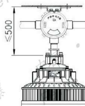
吊杆式(G)/配吊灯盒 Suspender type(G)/ equipment chandelier box
