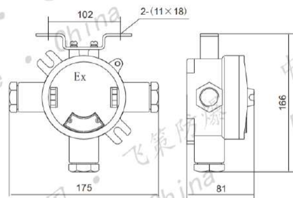
吊灯盒 SFH-20d Hanging box
