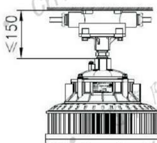
吸顶式(X)/配接线盒 Ceiling type(X)/ equipment junction box
