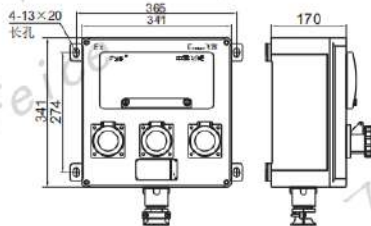
2型16A插销 2Type 16A latch
