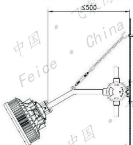
壁式30° (B1) / 配吊灯盒 Wall type 30° (B1) / equipment chandelier box
