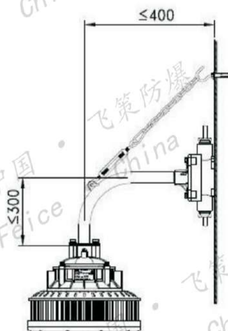
壁式90°(B2)/配接线盒 Wall type 90°(B2)/ equipment junction box
