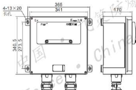
80A、100A小型断路器(3P/4P) 80A, 100A miniature circuit breaker (3P/4P)
