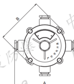
防爆接线盒配吊盖 (IIB/IIC) Explosion-proof hanging box
