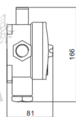
防爆吊灯盒 (IIB/IIC) Explosion-proof hanging box
