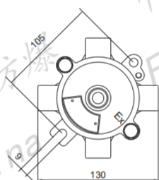
防爆接线盒 (e) Explosion-proof junction box (e)
