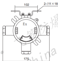
防爆接线盒配吊盖 (IIB/IIC) Explosion-proof hanging box
