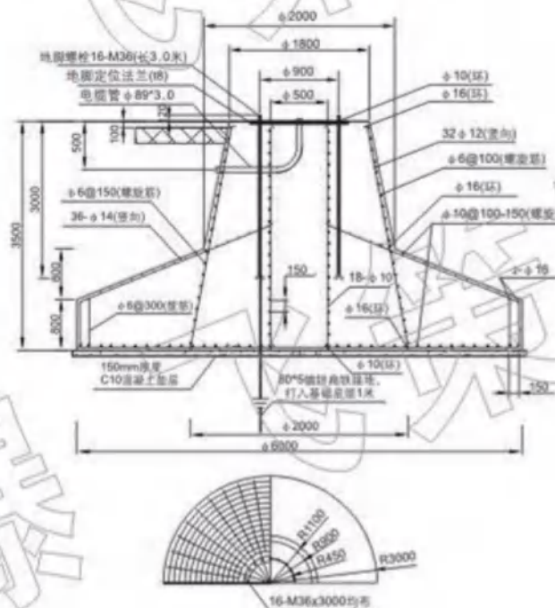
35m高杆灯 High-pole lamp 基础平面图 Foundation plan
