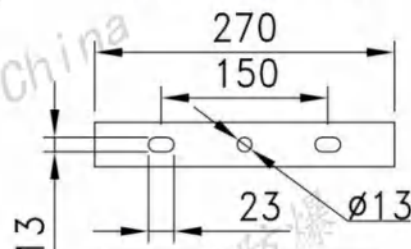
III型吸顶或壁式 Type III ceiling or wall type
