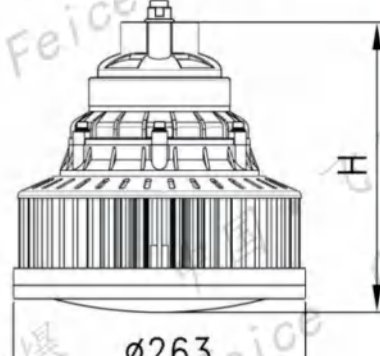
III型吸顶或壁式 Type III ceiling or wall type
