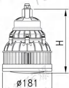
I型吸顶或壁式 Type I ceiling or wall type
