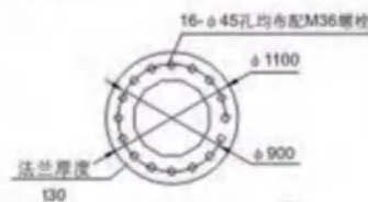
Flange plane schemes
