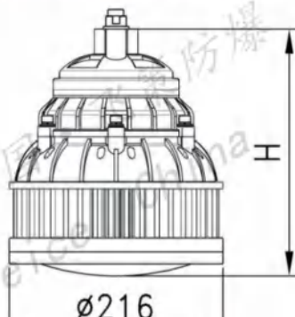
II型吸顶或壁式 Type II ceiling or wall type
