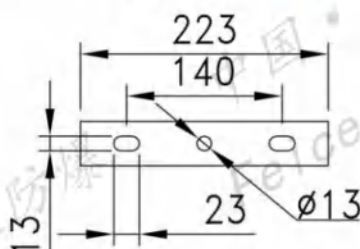
II型吸顶或壁式 Type II ceiling or wall type
