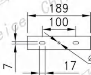
I型吸顶或壁式 Type I ceiling or wall type
