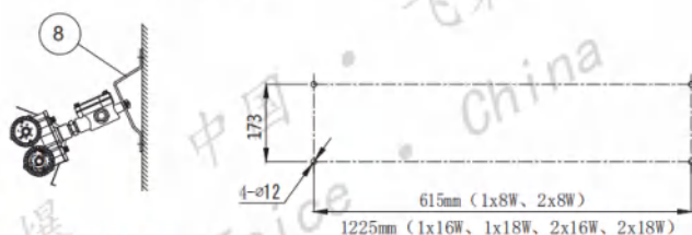
壁式30° B1 Wall type 30°
